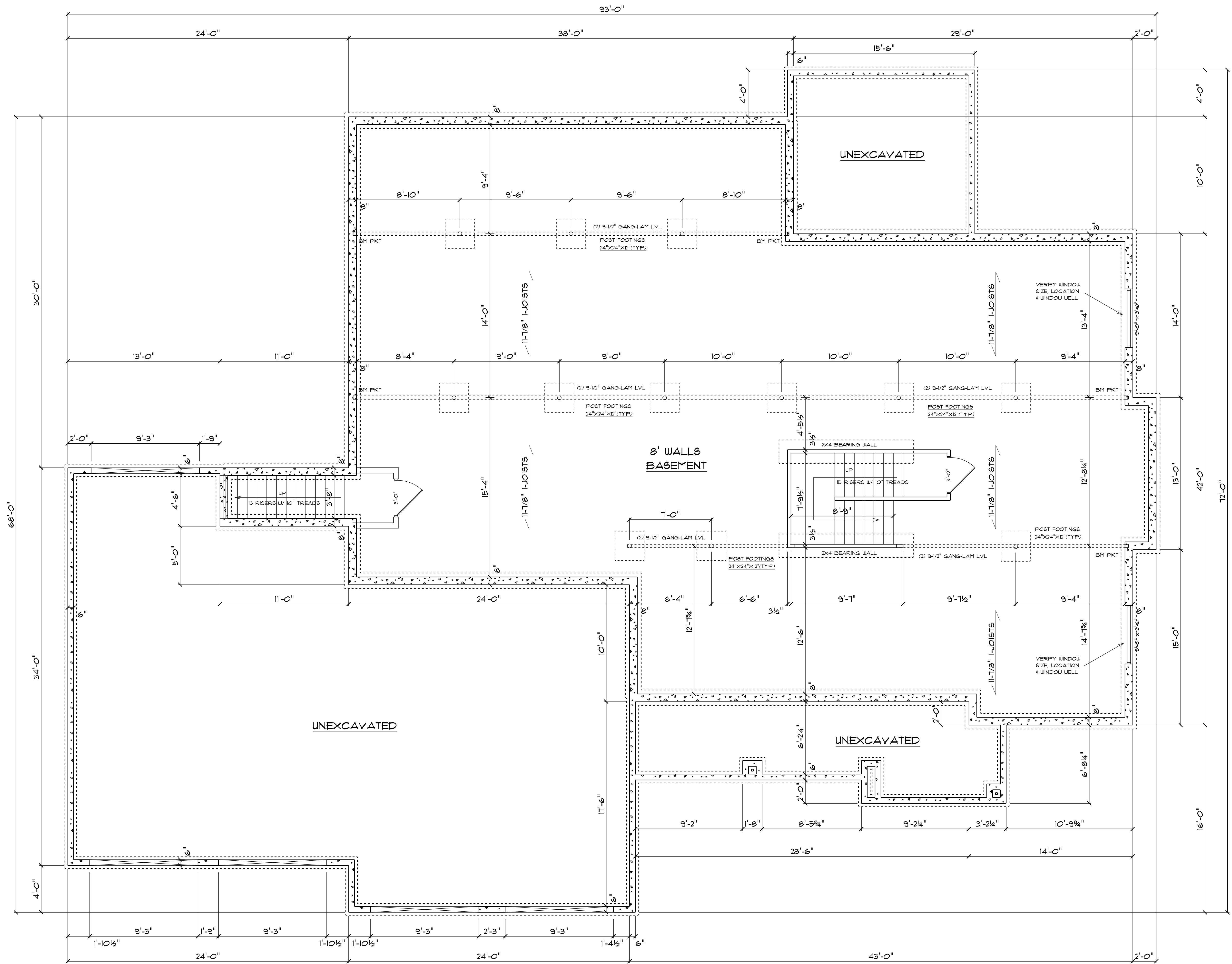
FOUNDATION PLAN
