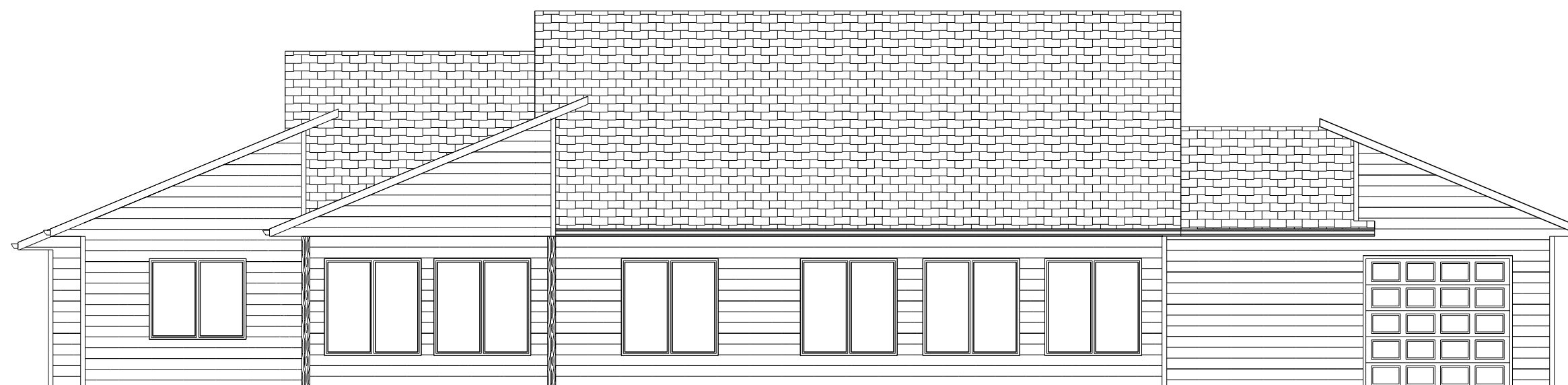
REAR ELEVATION
